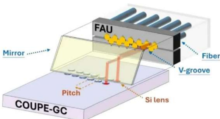
Grating Coupling FAU
