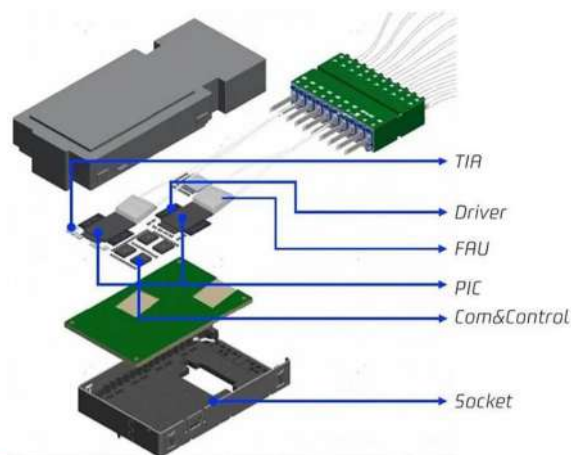
CW Laser Based NPO
